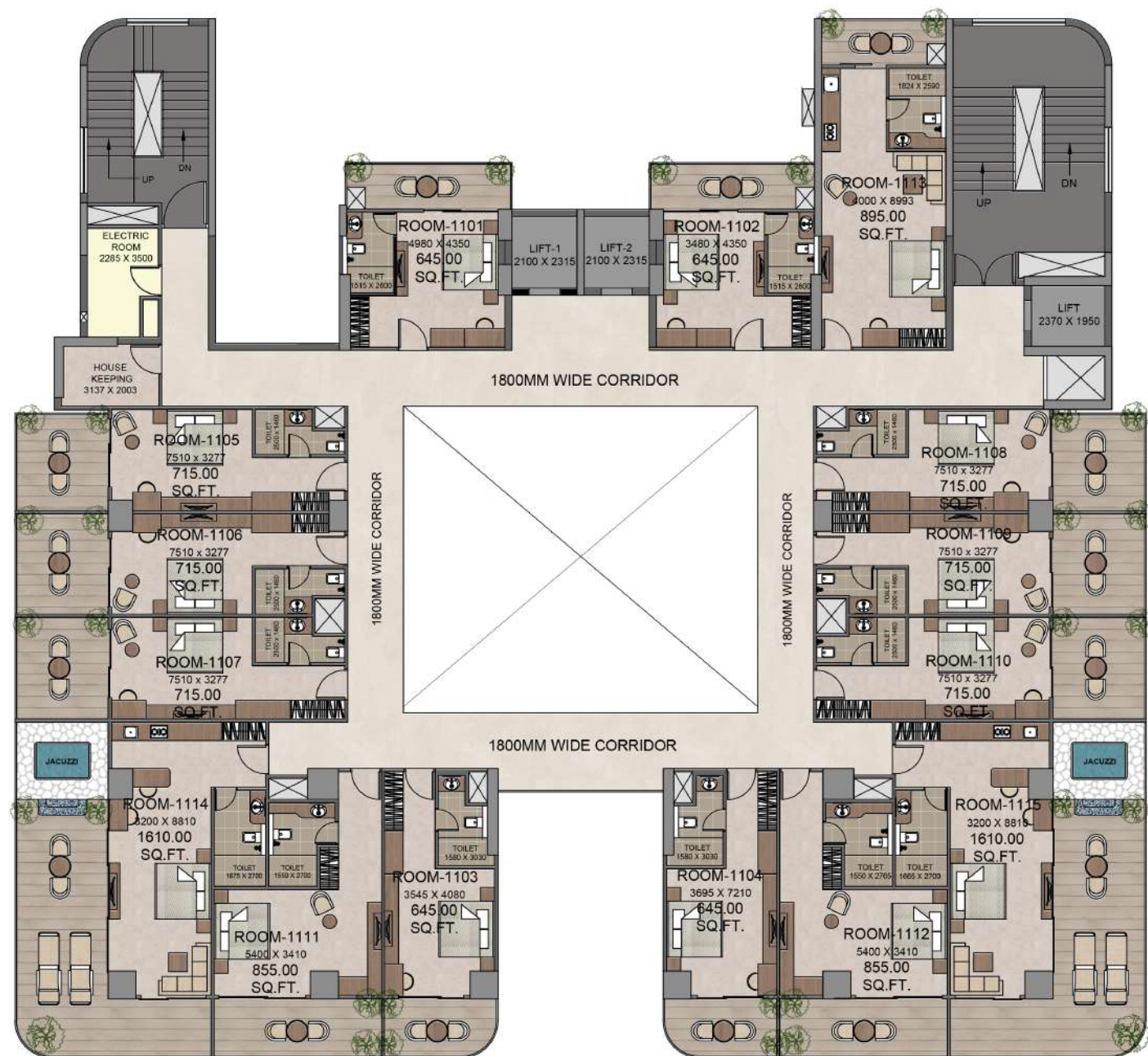
11TH - 16TH FLOOR PLAN
