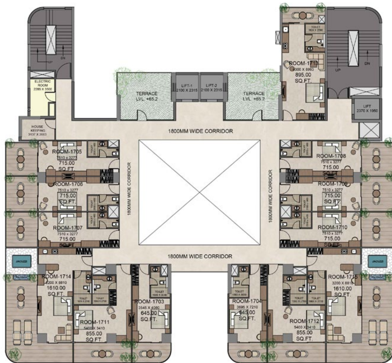
17TH FLOOR PLAN
