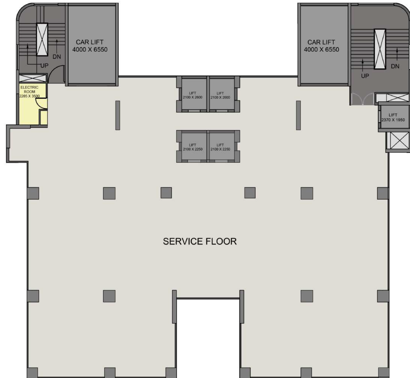
8TH FLOOR PLAN
