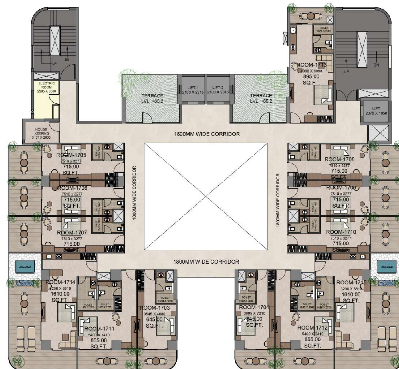
17TH FLOOR PLAN
